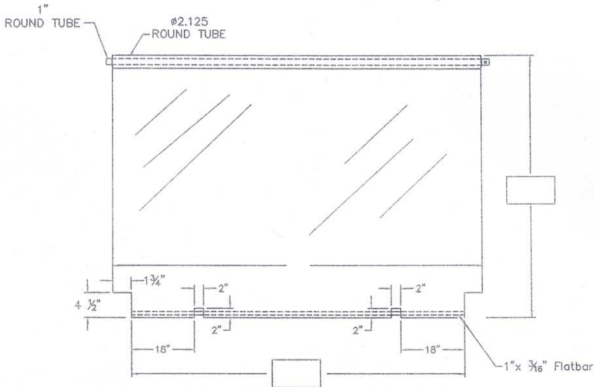
STANDARD UNIT DETAIL PLAN VIEW
